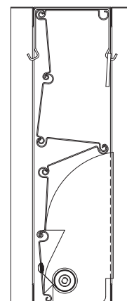
Closed Position (D17V)
